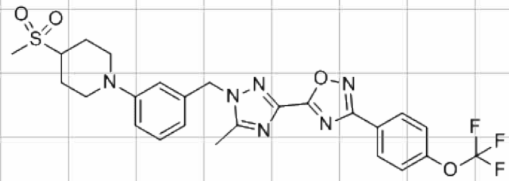
PC-3520501, CDCl 3
